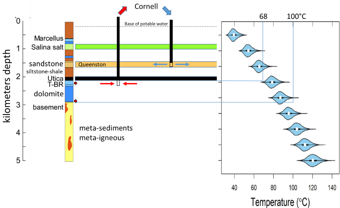
Figure 1. Cartoon illustration of stratigraphy under the Cornell campus adapted from figures from (Gustafson et al. 2018). The two most promising intervals for ESH production are vertically fractured grabens in the Trenton-Black River (T-BR) and sand and gravel filled paleo-valleys on top of basement, indicated by small red arrows outlined in black next to the stratigraphic column. Pore waters are generally brines below ~300 m (dashed black line).
